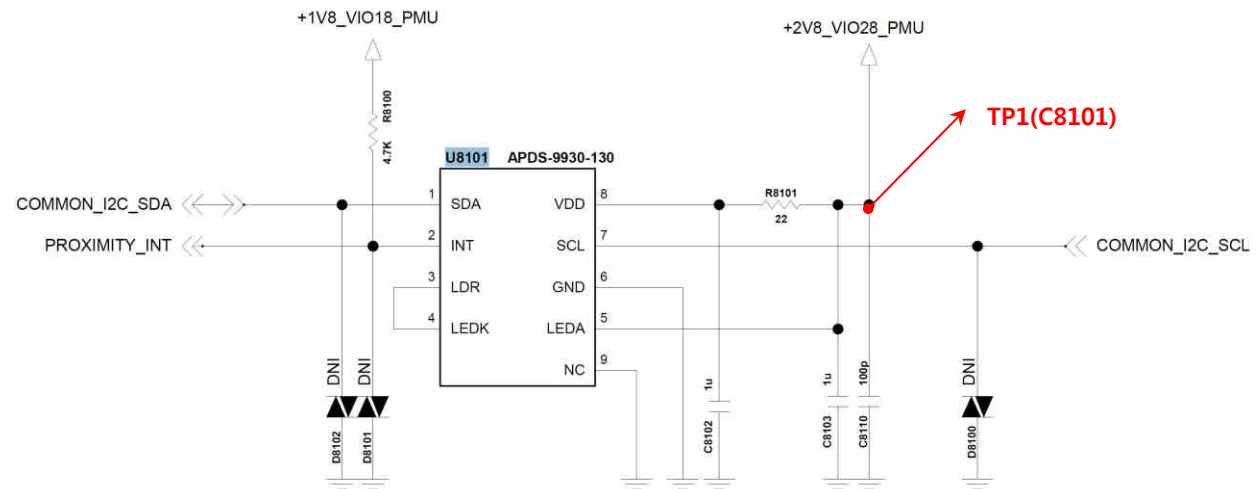
Circuit Diagram
