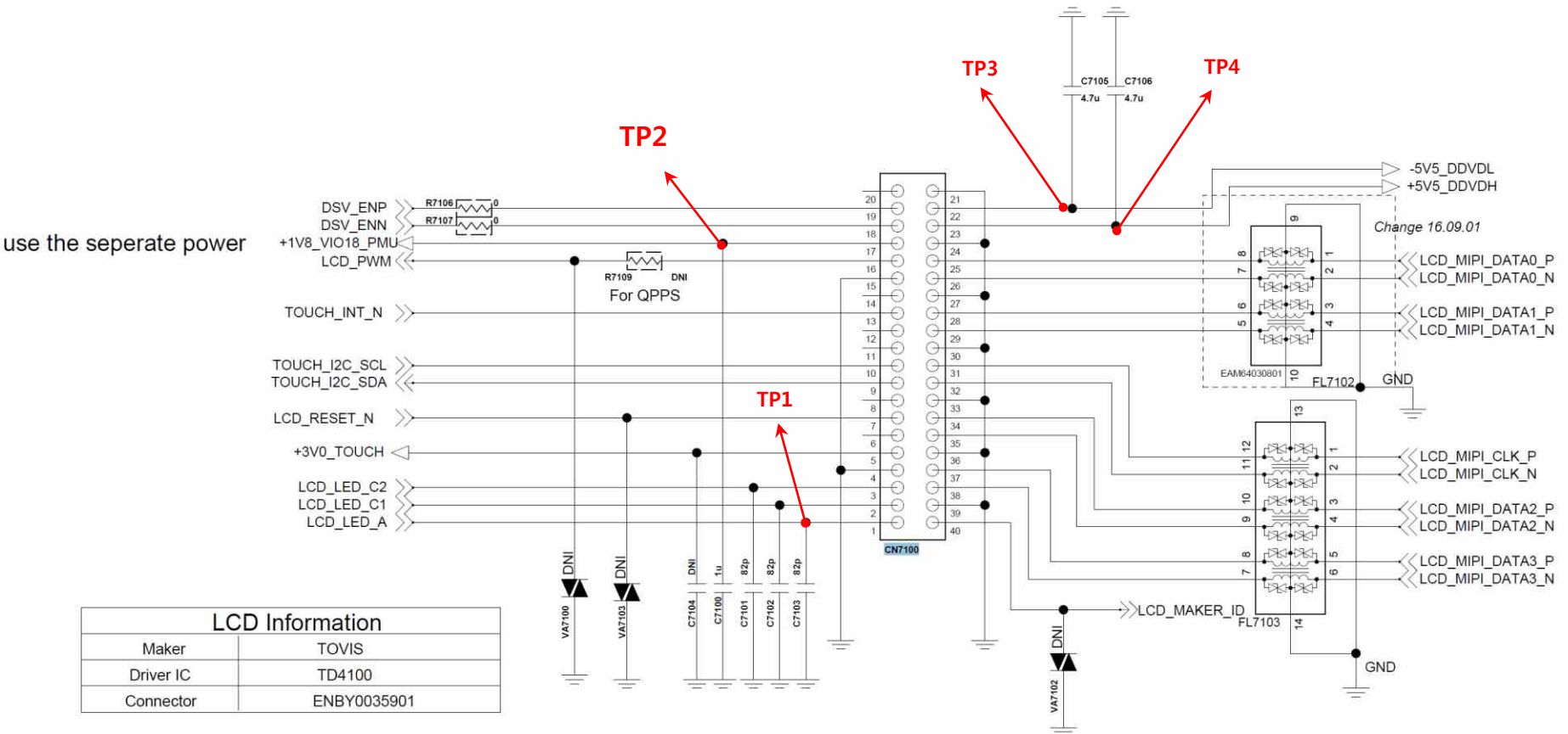
Circuit Diagram
