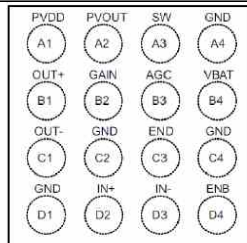
U6610_TPA2015D1, IC, Speaker AMP (Top View)
